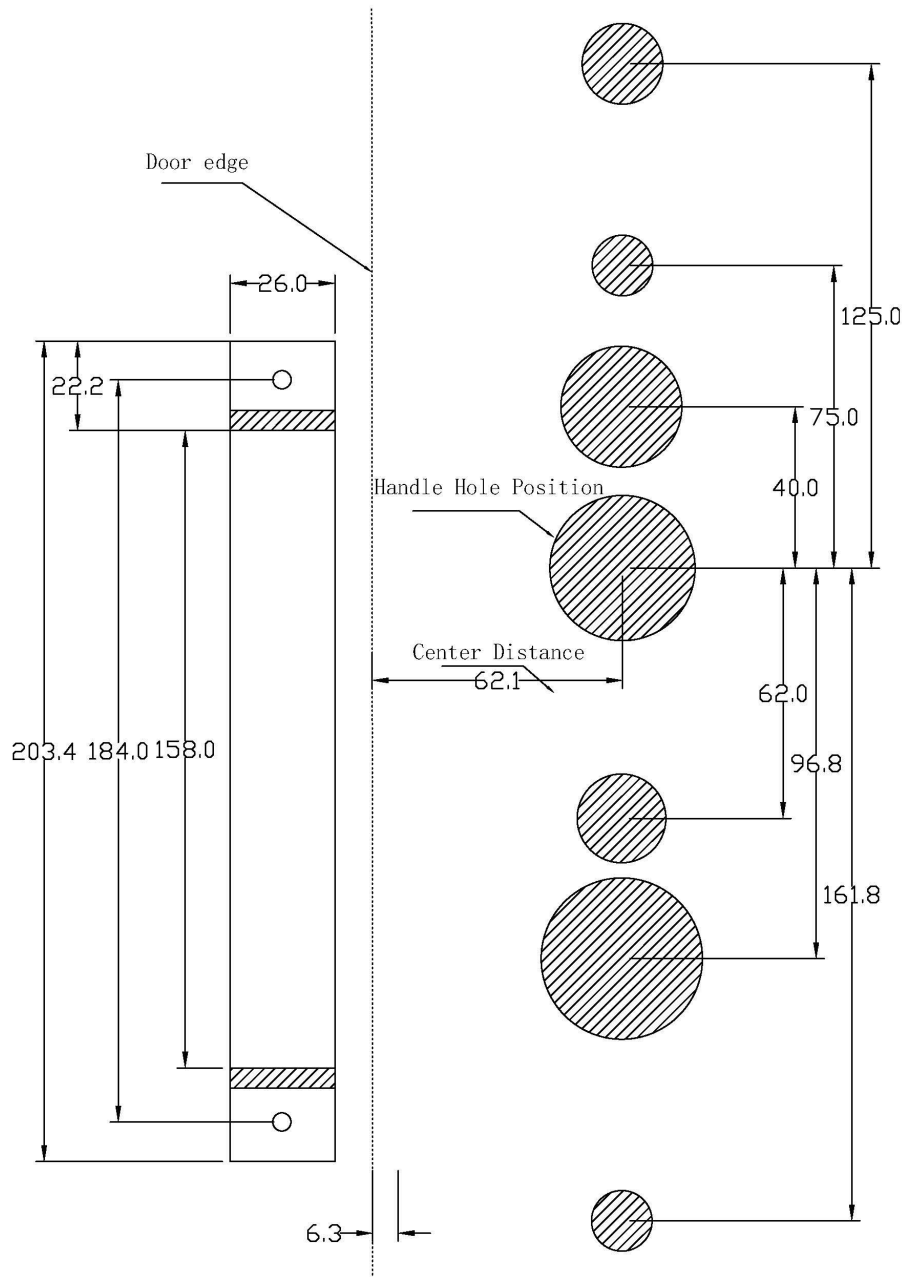
SL-HD2&D3 Lock Mortise Drilling Template (2#DS Lock Mortise)
